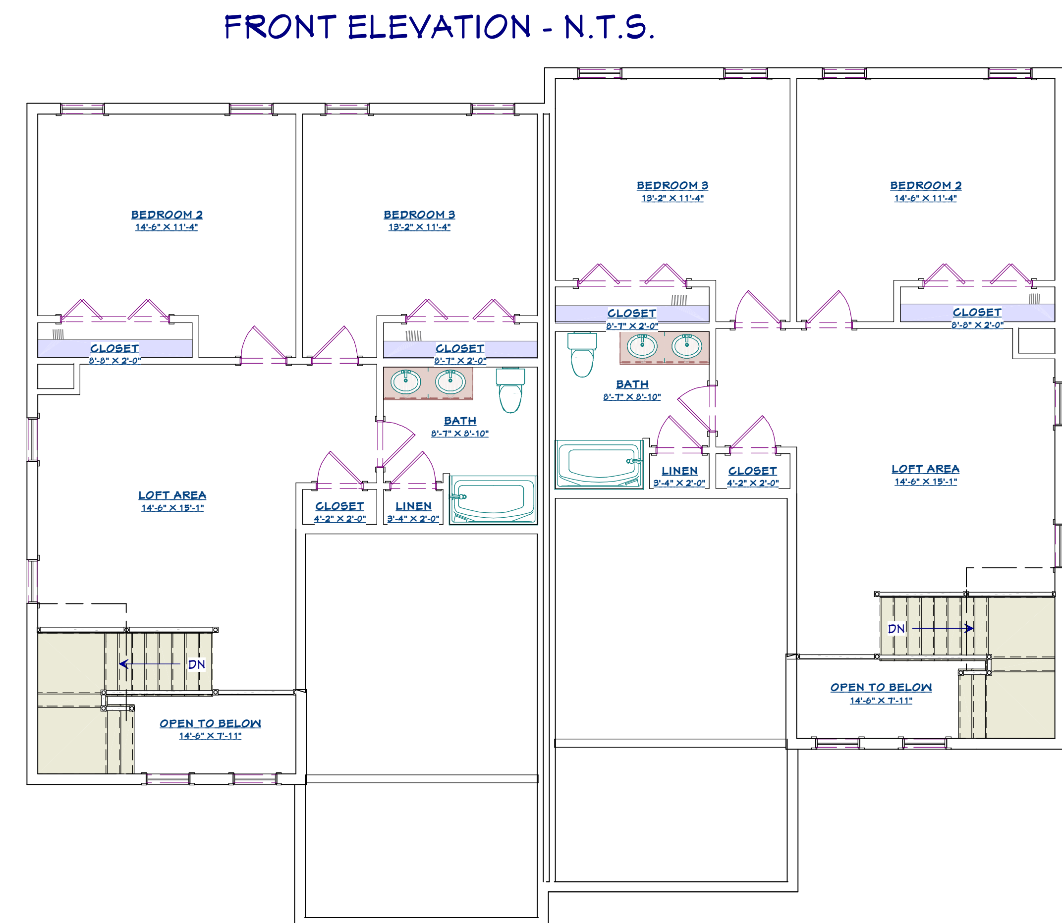
PROPOSED SECOND FLOOR PLAN - N.T.S.
