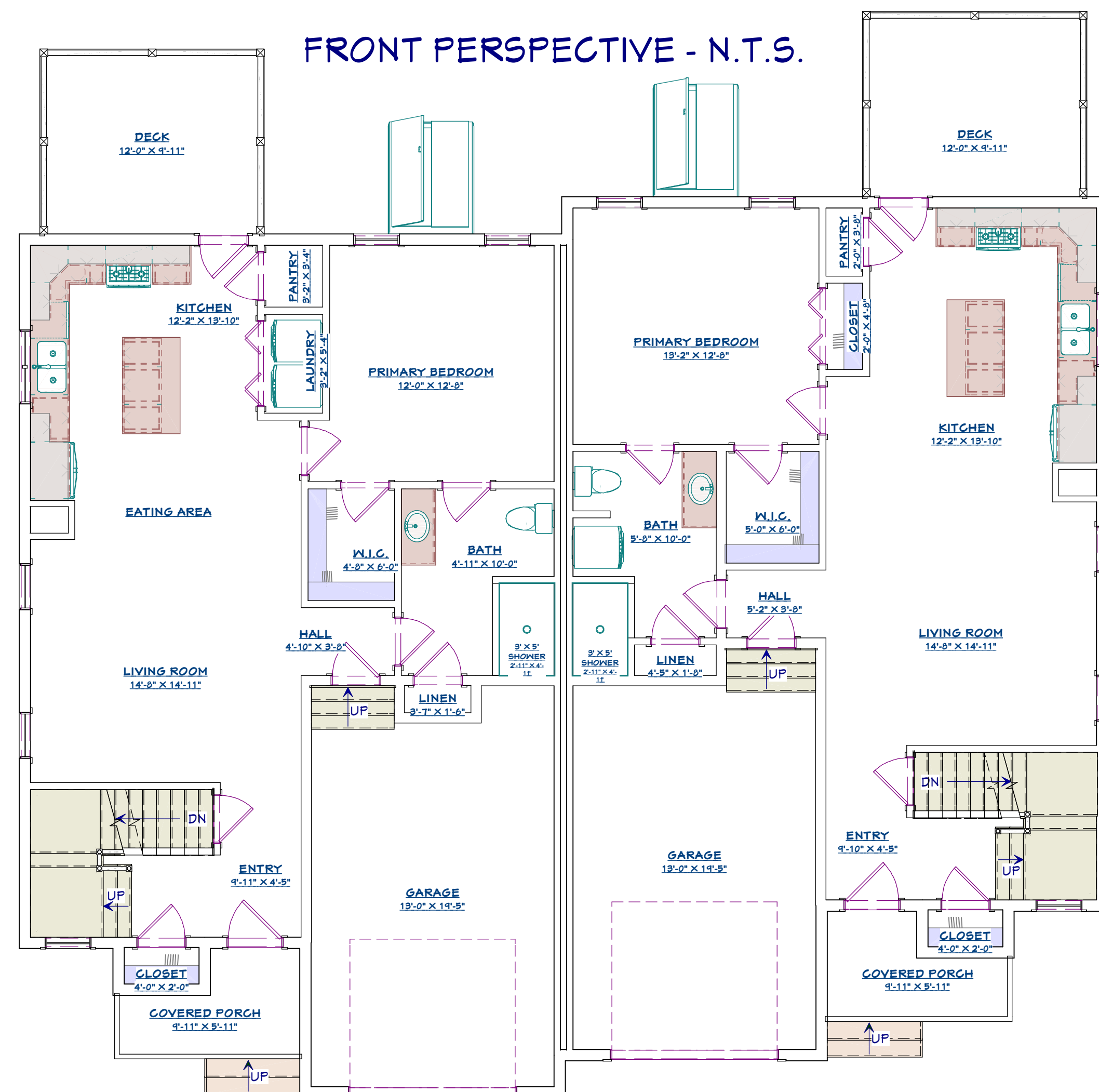
PROPOSED FIRST FLOOR PLAN - N.T.S.
